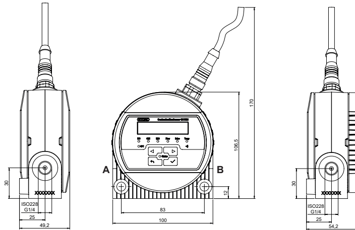
Flange connection
